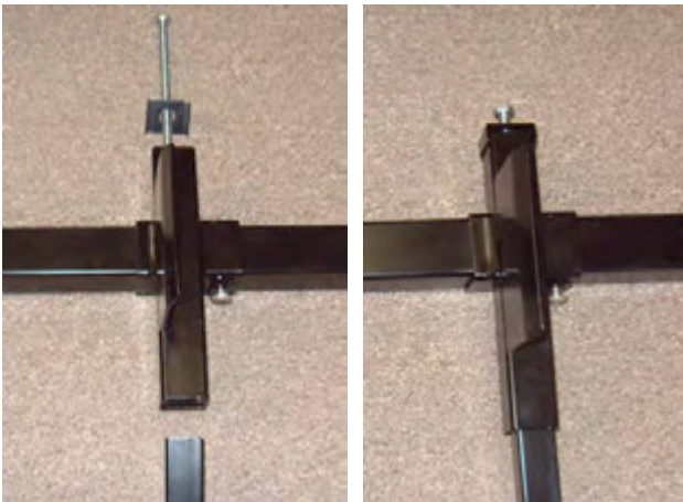
Figs 4. & 5. Wheel chock and receiver during assembly Fig 6. Mounted rack with wheel in webbing of wheel chock
