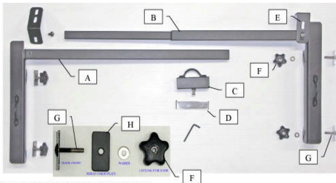
FIG. 1 Basic Rack for Truck Beds with Track Systems.
