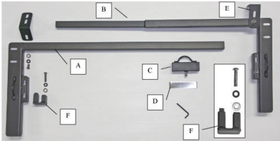
FIG. 1 Basic Rack for Fleetside Beds
